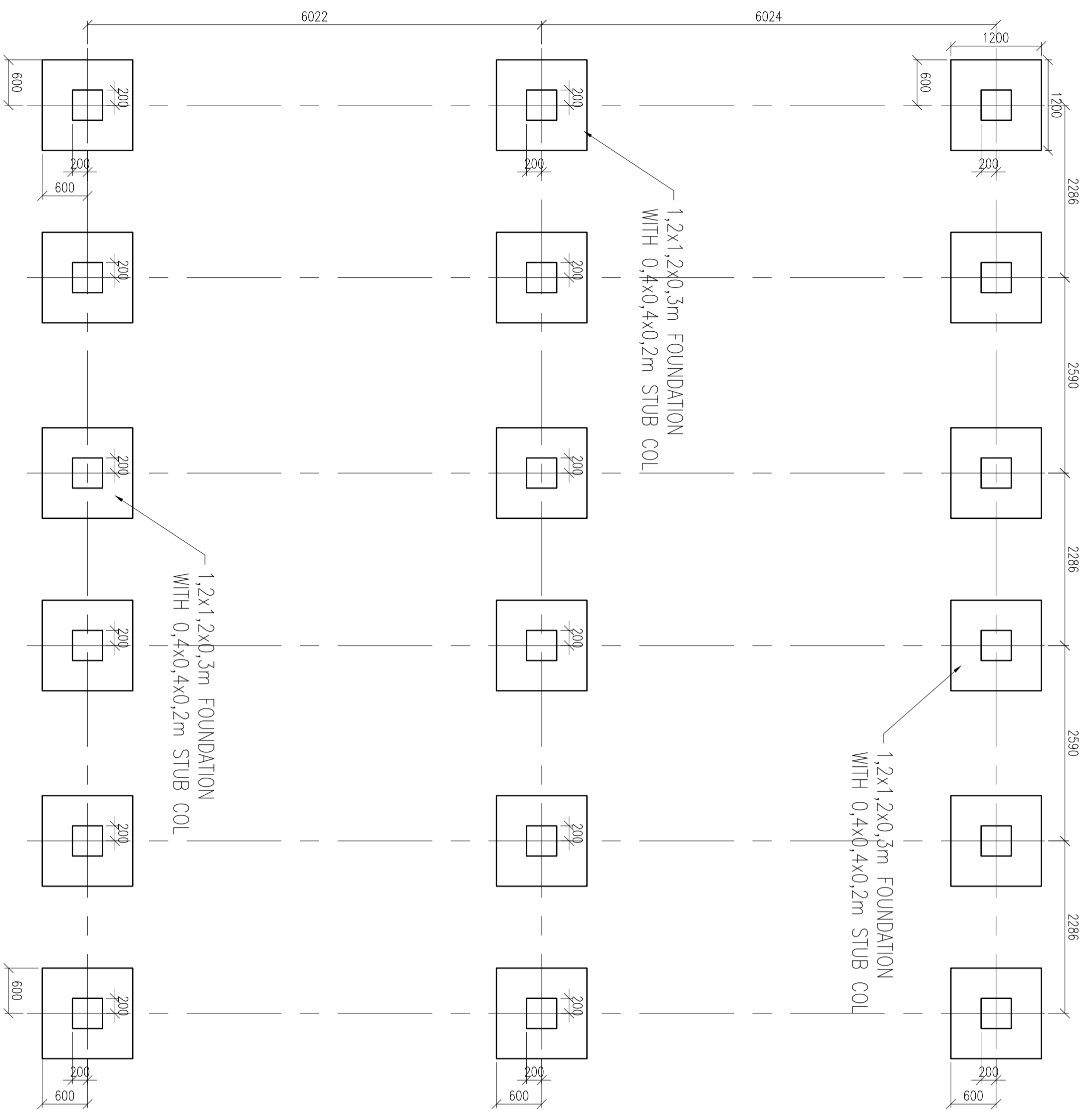
LAYOUT SCALE 1:50
