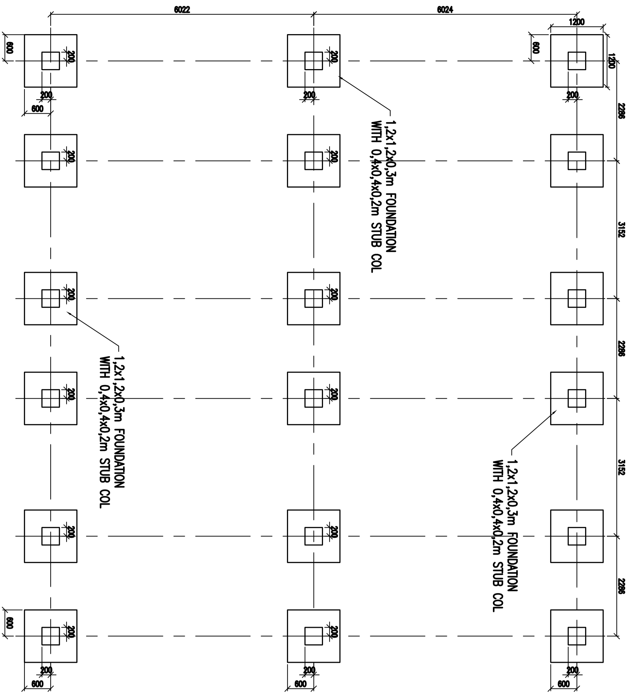
LAYOUT SCALE 1:50
