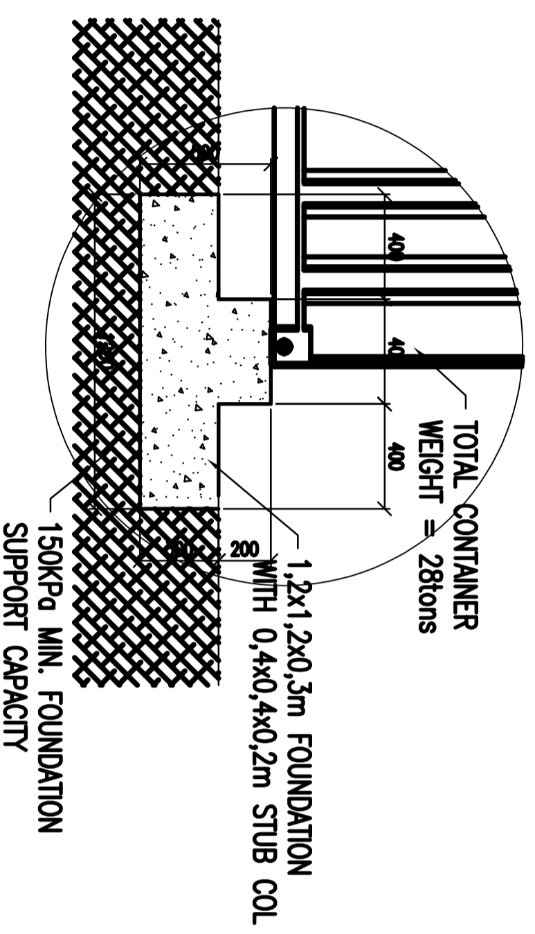
SECTION SCALE 1:20
